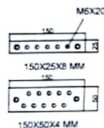
DETAILS OF BUSBAR CONNECTION
